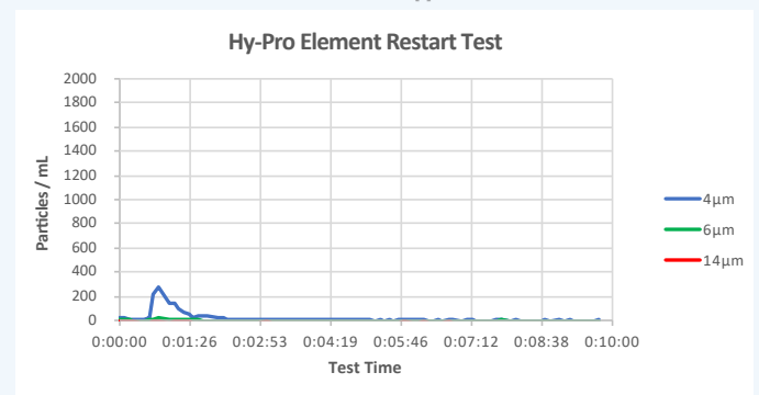
Figure 9: Hy-Pro DFE Restart Test
